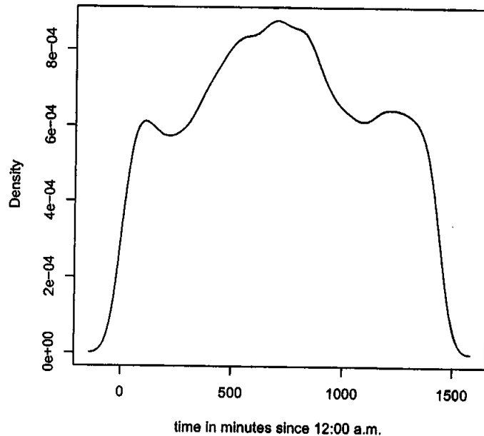
Fig. 4. Kernel estimate of time-of-day density.
