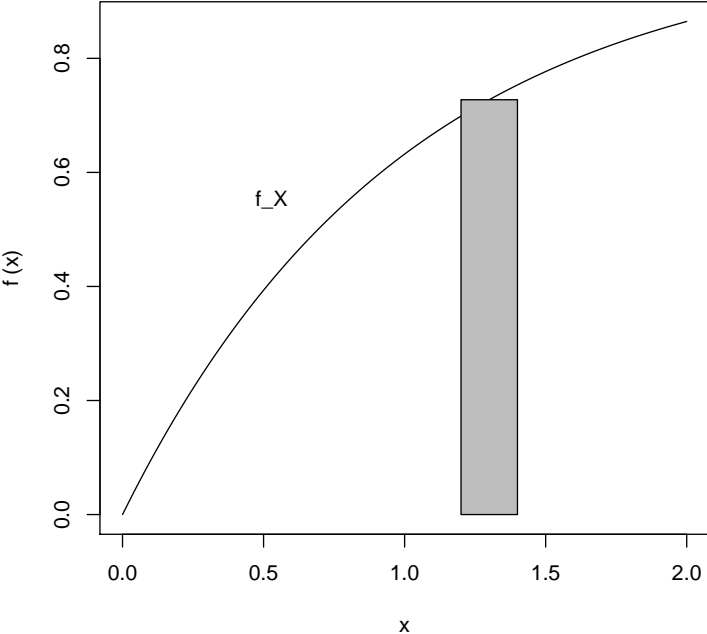
Figure 7.1: Approximation of Probability by a Rectangle
